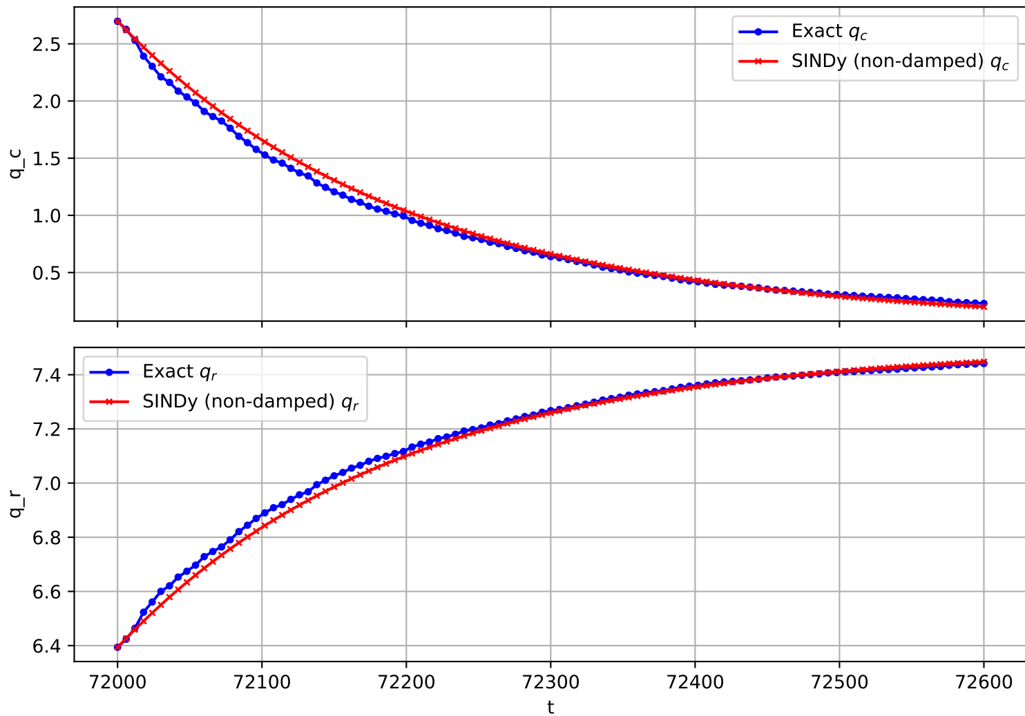
Trajectory 1352 (non-damped)
