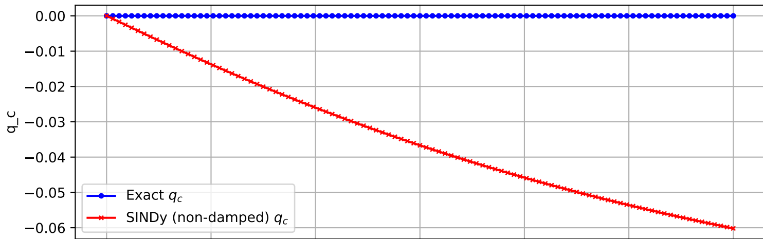
Trajectory 1360 (non-damped)
