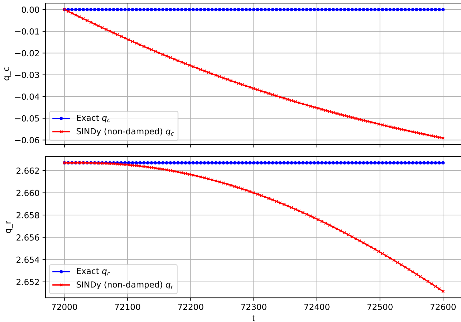
Trajectory 1362 (non-damped)
