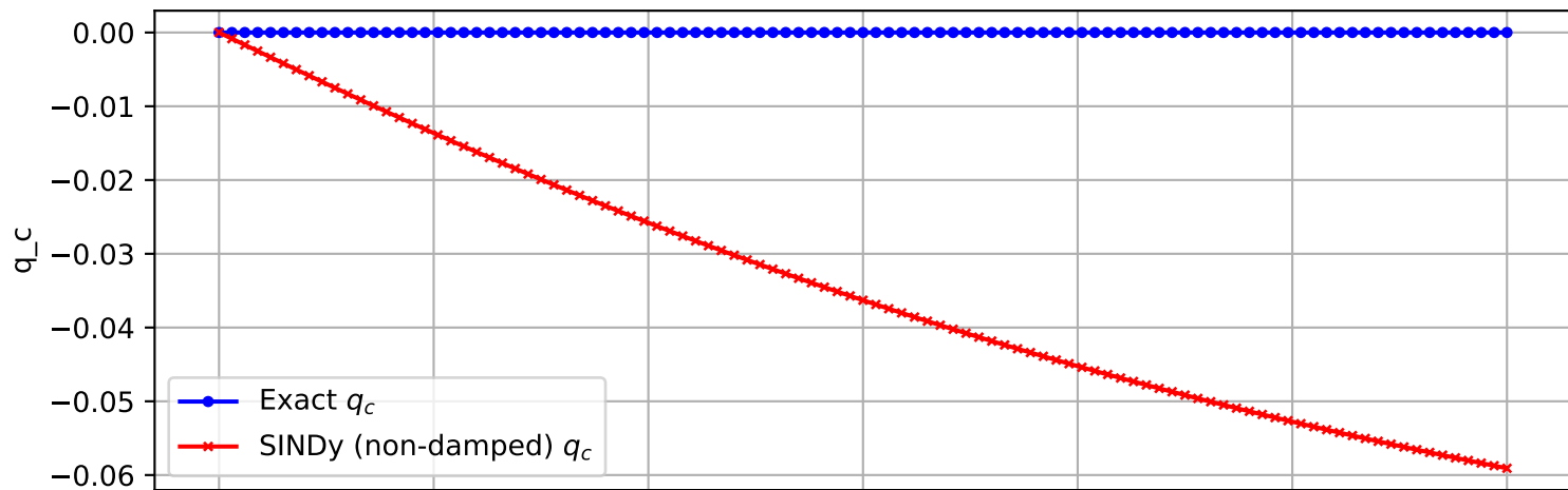
Trajectory 1364 (non-damped)
