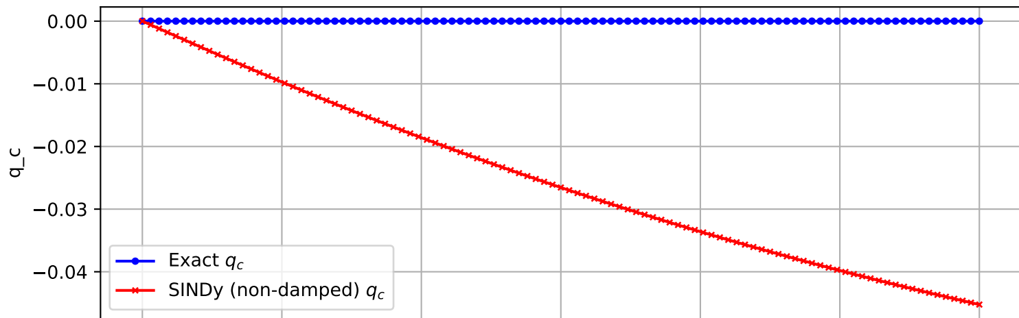
Trajectory 1368 (non-damped)
