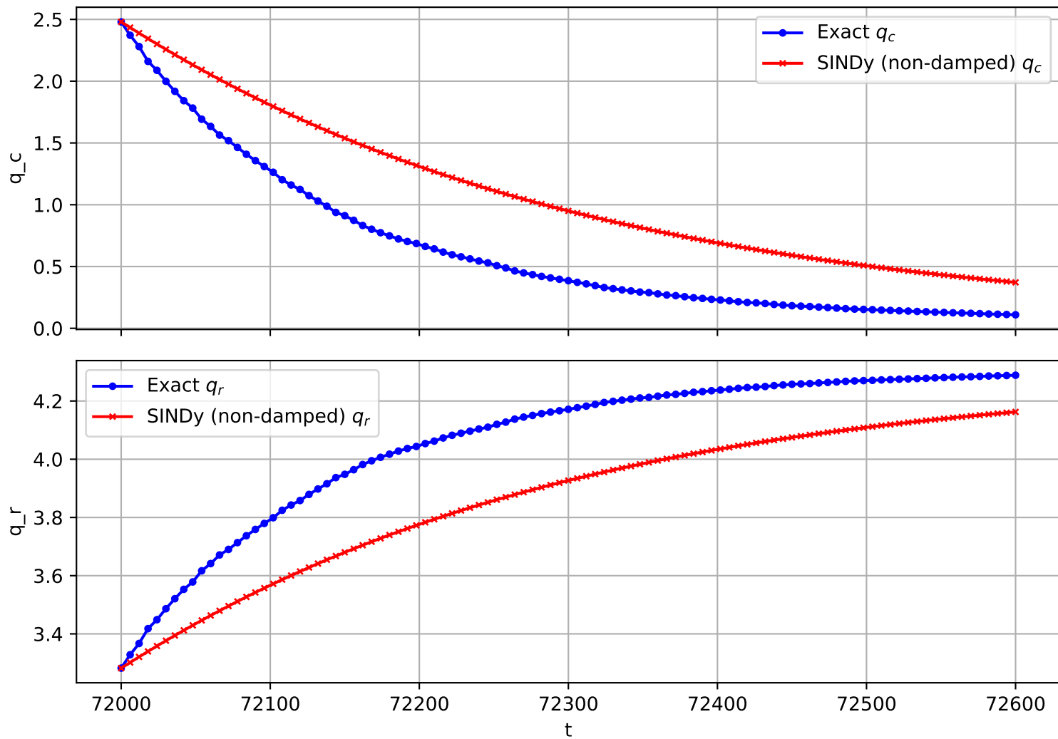
Trajectory 1374 (non-damped)
