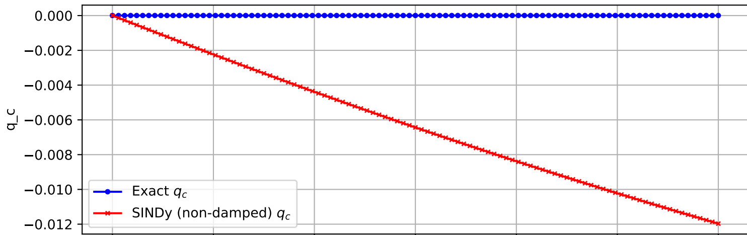
Trajectory 1378 (non-damped)
