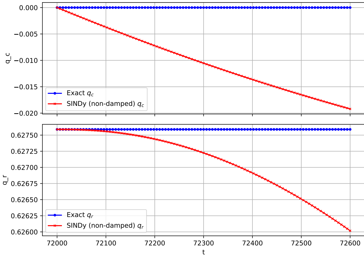
Trajectory 1380 (non-damped)
