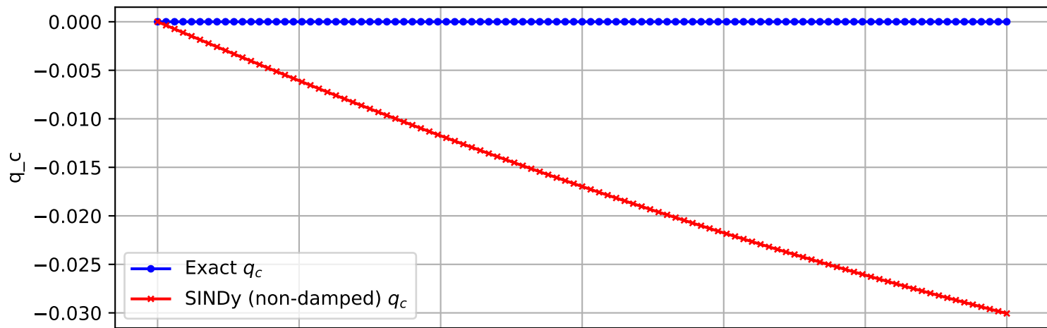
Trajectory 1385 (non-damped)
