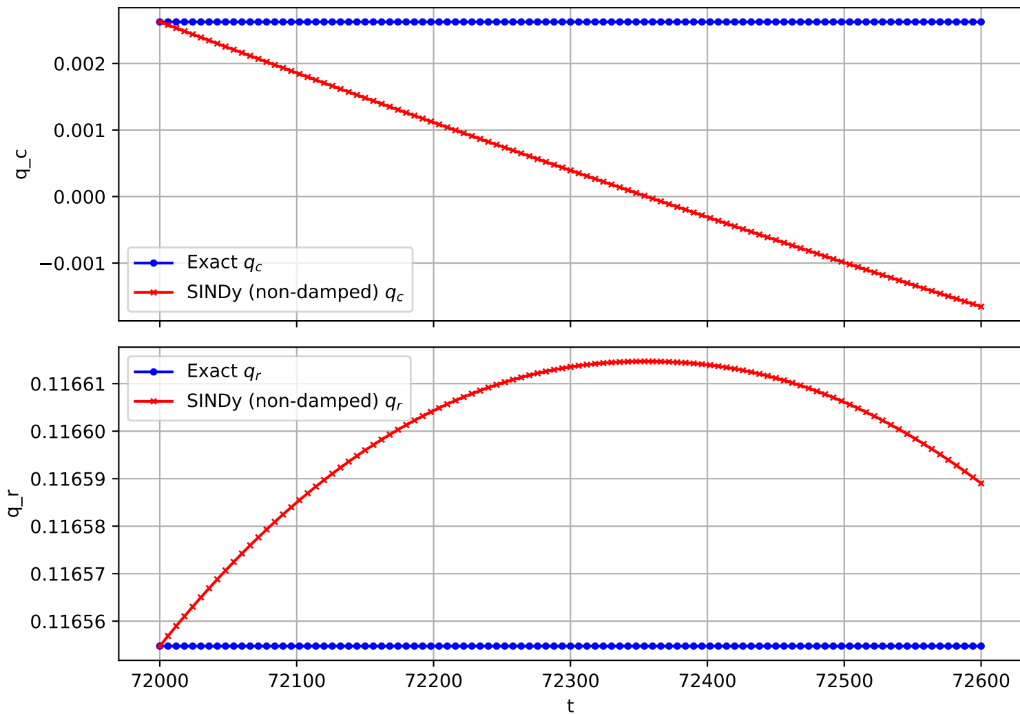
Trajectory 1396 (non-damped)
