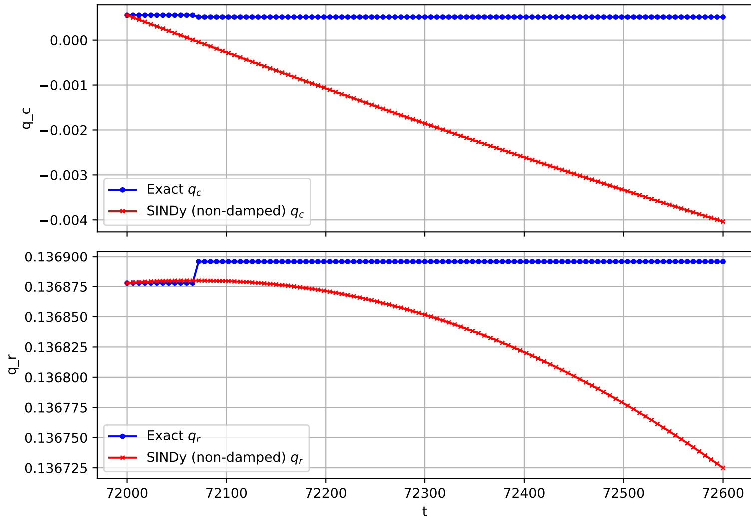
Trajectory 1400 (non-damped)
