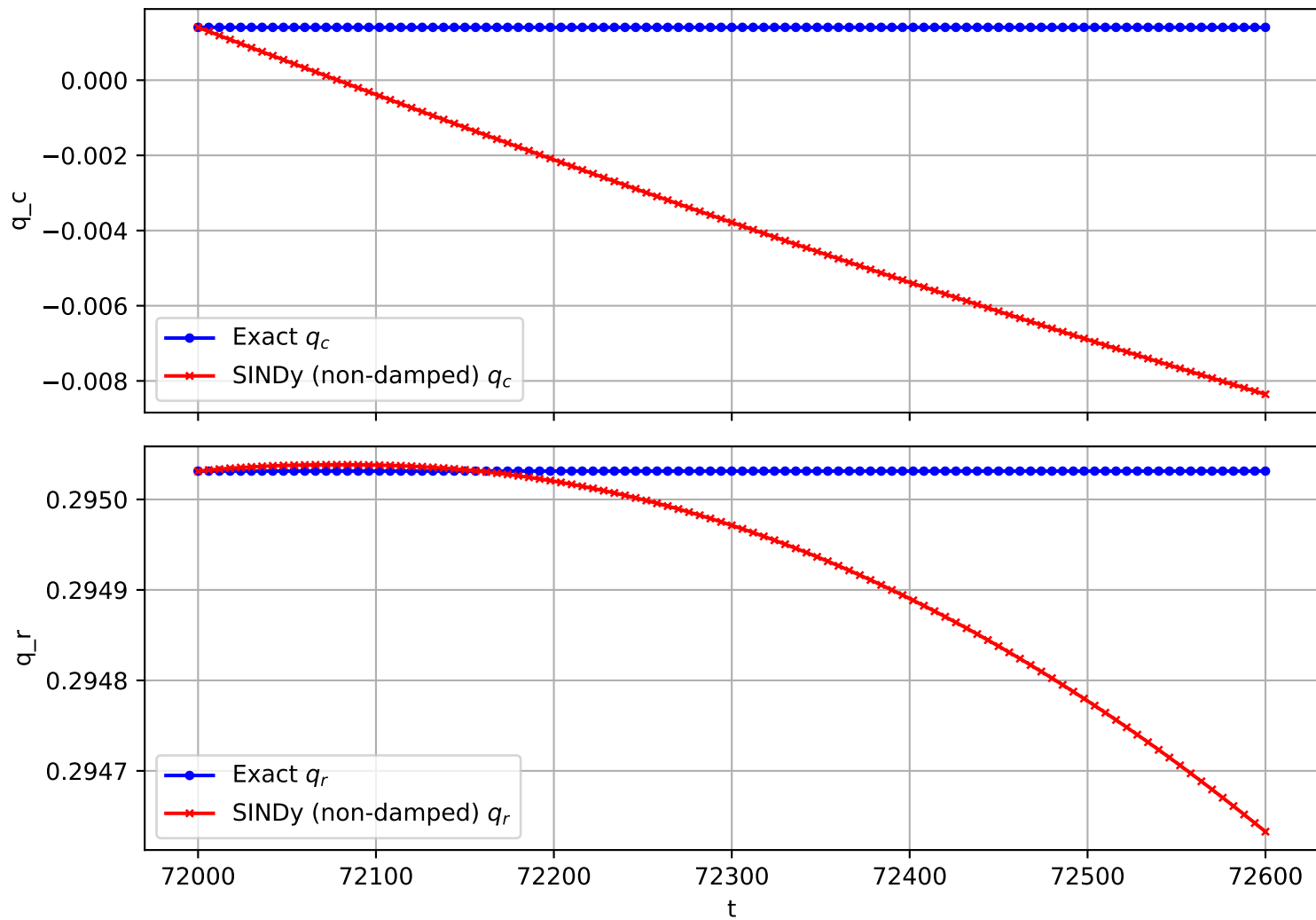
Trajectory 1401 (non-damped)
