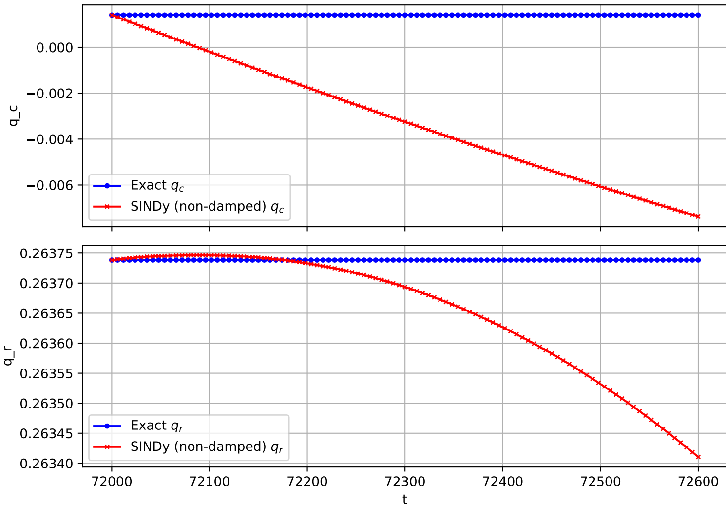
Trajectory 1402 (non-damped)
