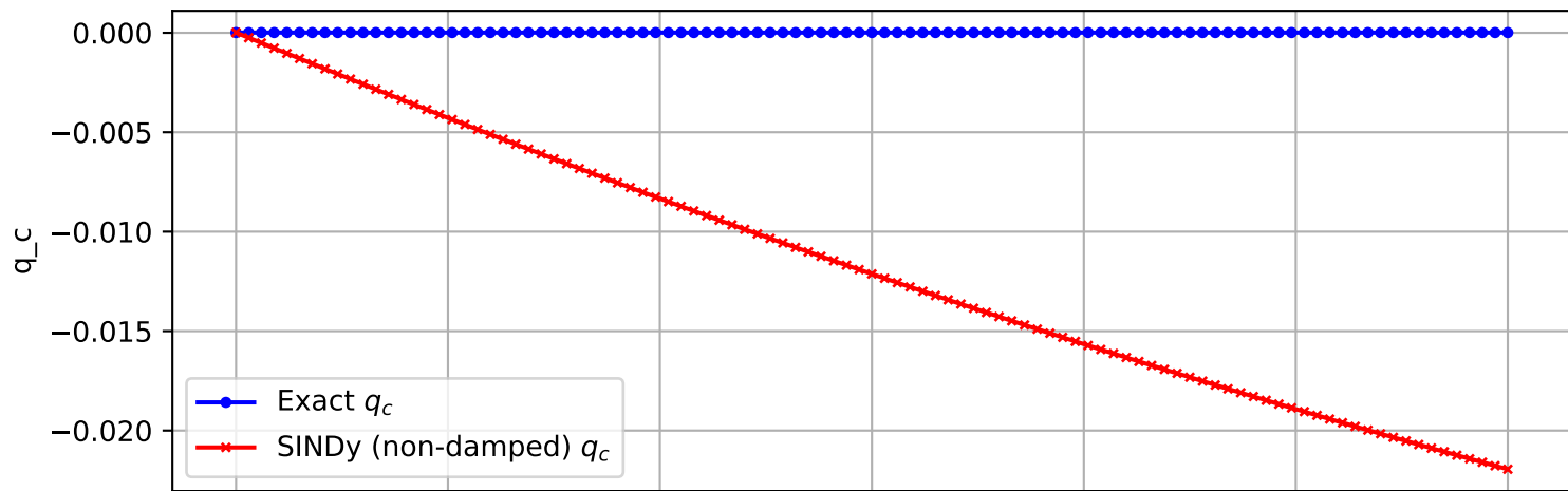
Trajectory 141 (non-damped)
