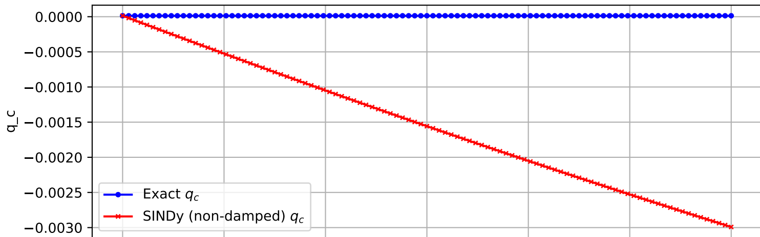
Trajectory 1413 (non-damped)
