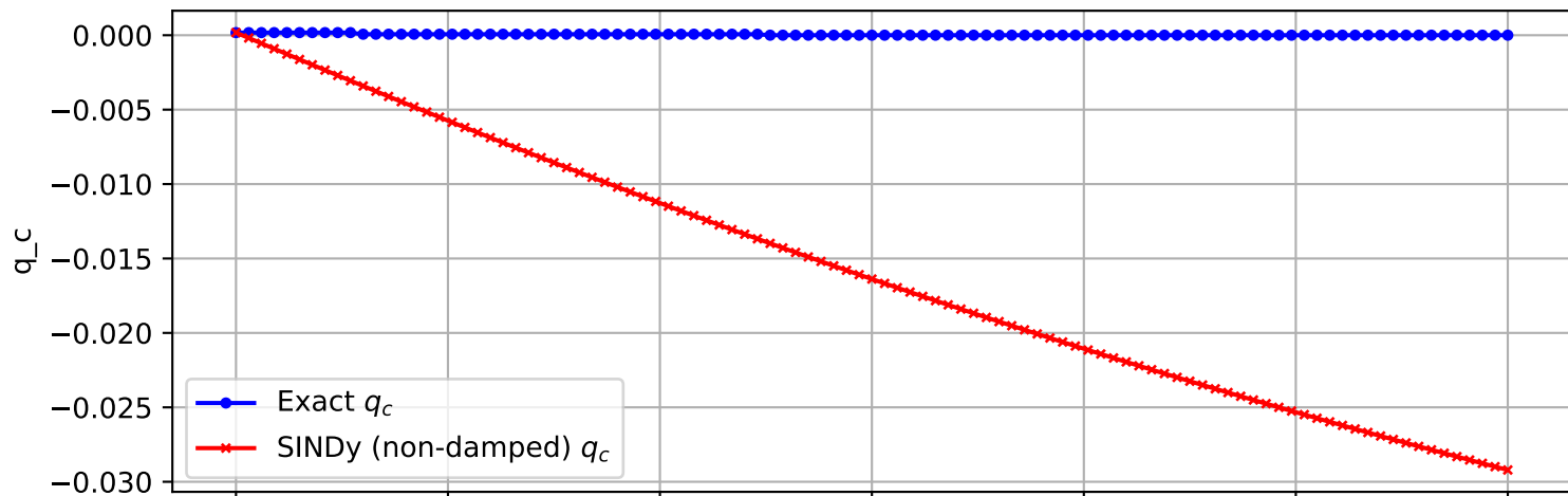
Trajectory 1426 (non-damped)
