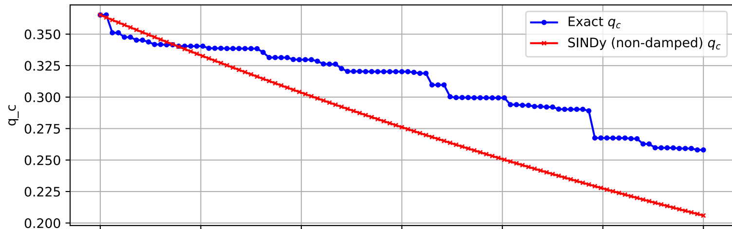
Trajectory 1428 (non-damped)
