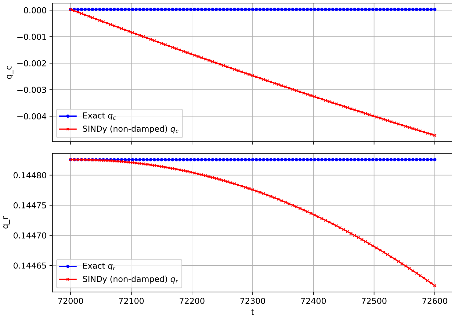
Trajectory 1432 (non-damped)
