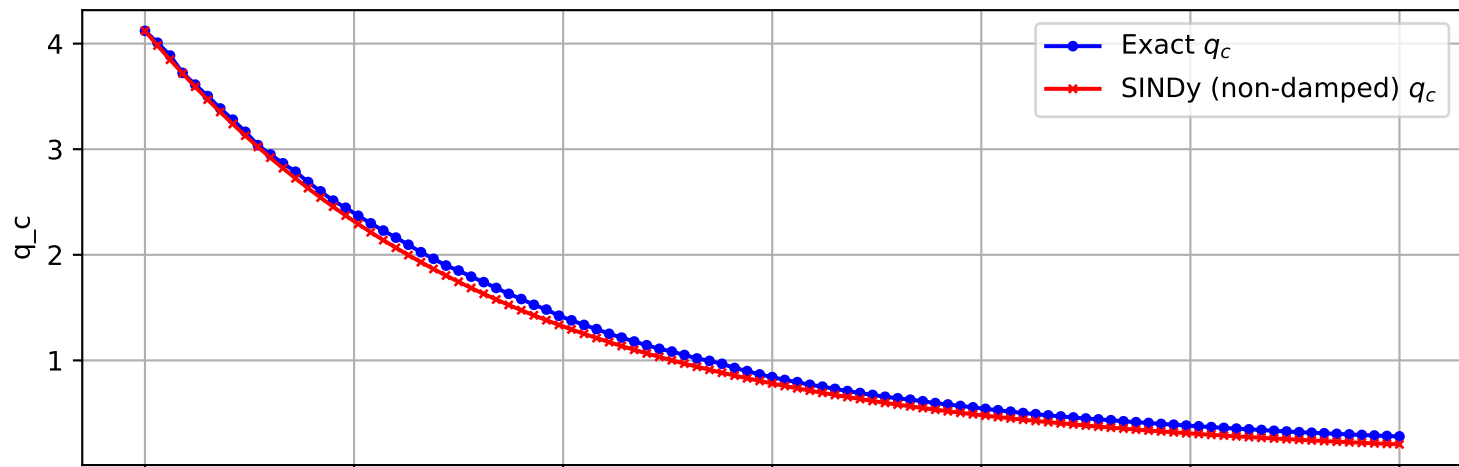
Trajectory 1436 (non-damped)
