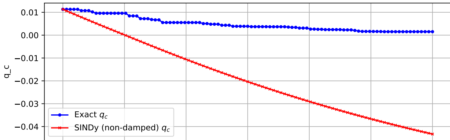
Trajectory 1440 (non-damped)
