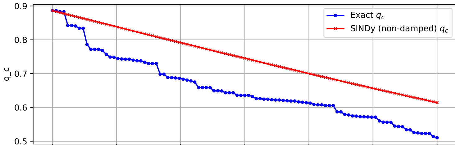
Trajectory 1459 (non-damped)
