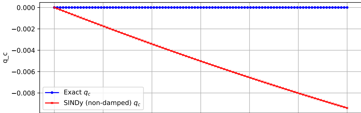
Trajectory 1464 (non-damped)
