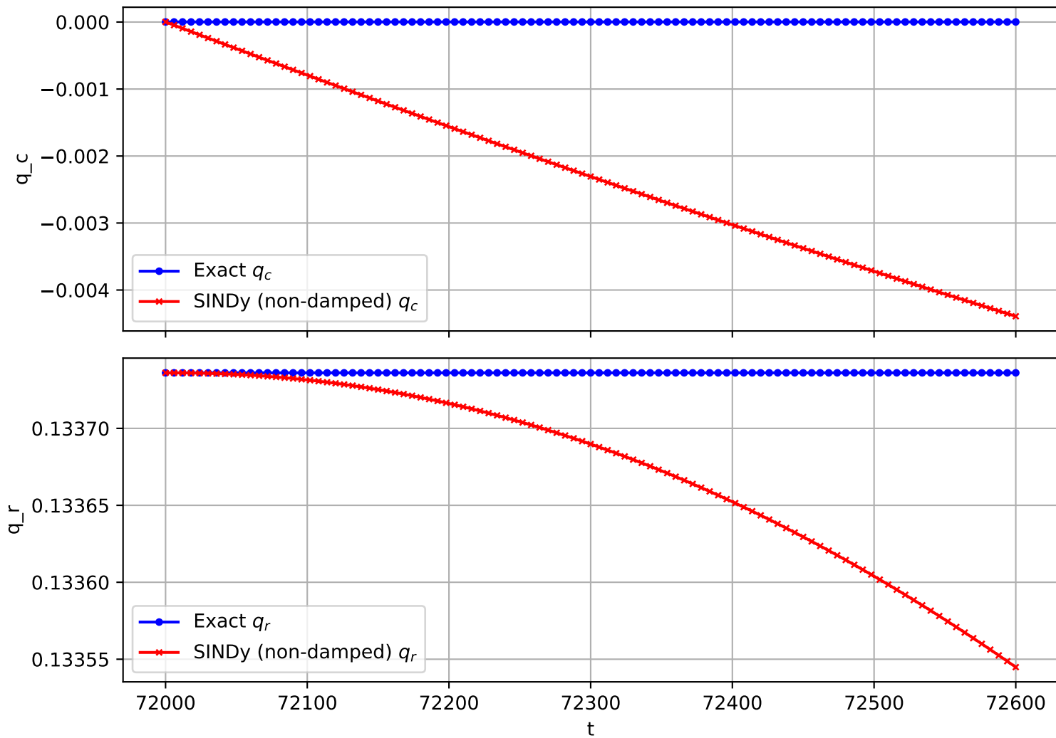
Trajectory 1469 (non-damped)
