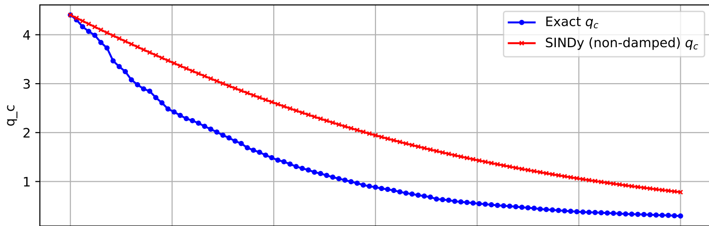
Trajectory 147 (non-damped)
