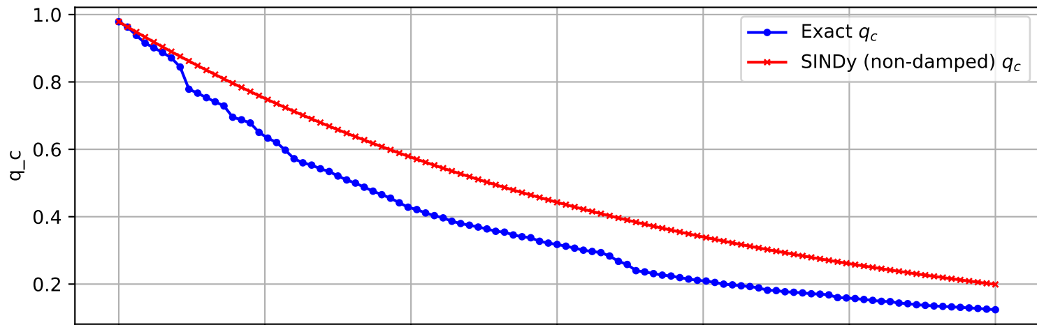
Trajectory 1475 (non-damped)
