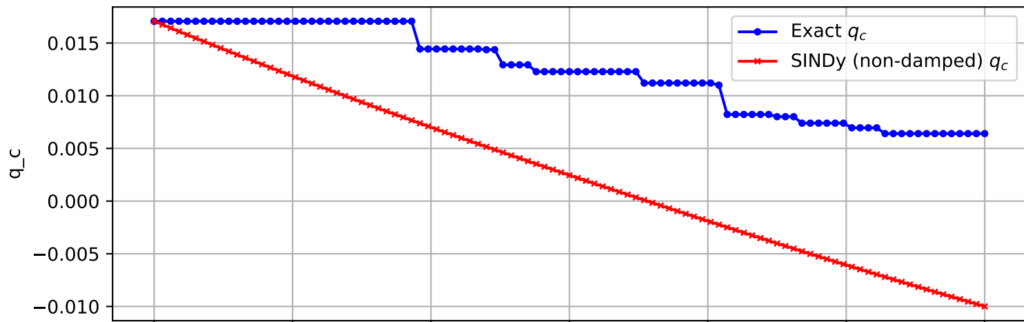
Trajectory 1483 (non-damped)
