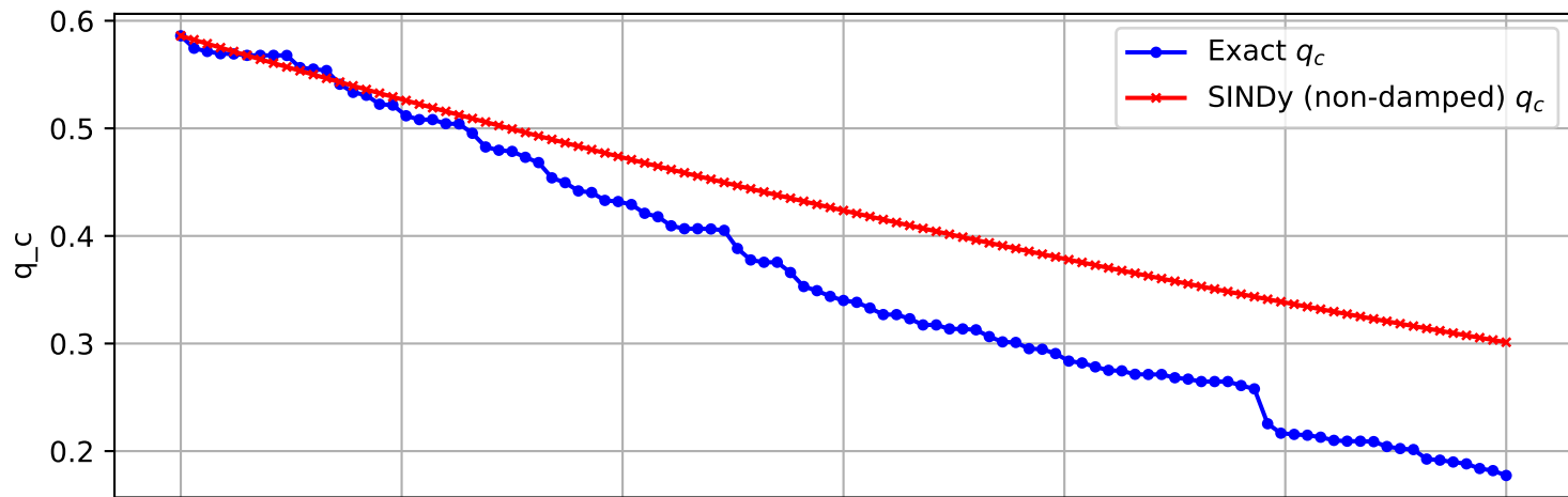
Trajectory 1485 (non-damped)
