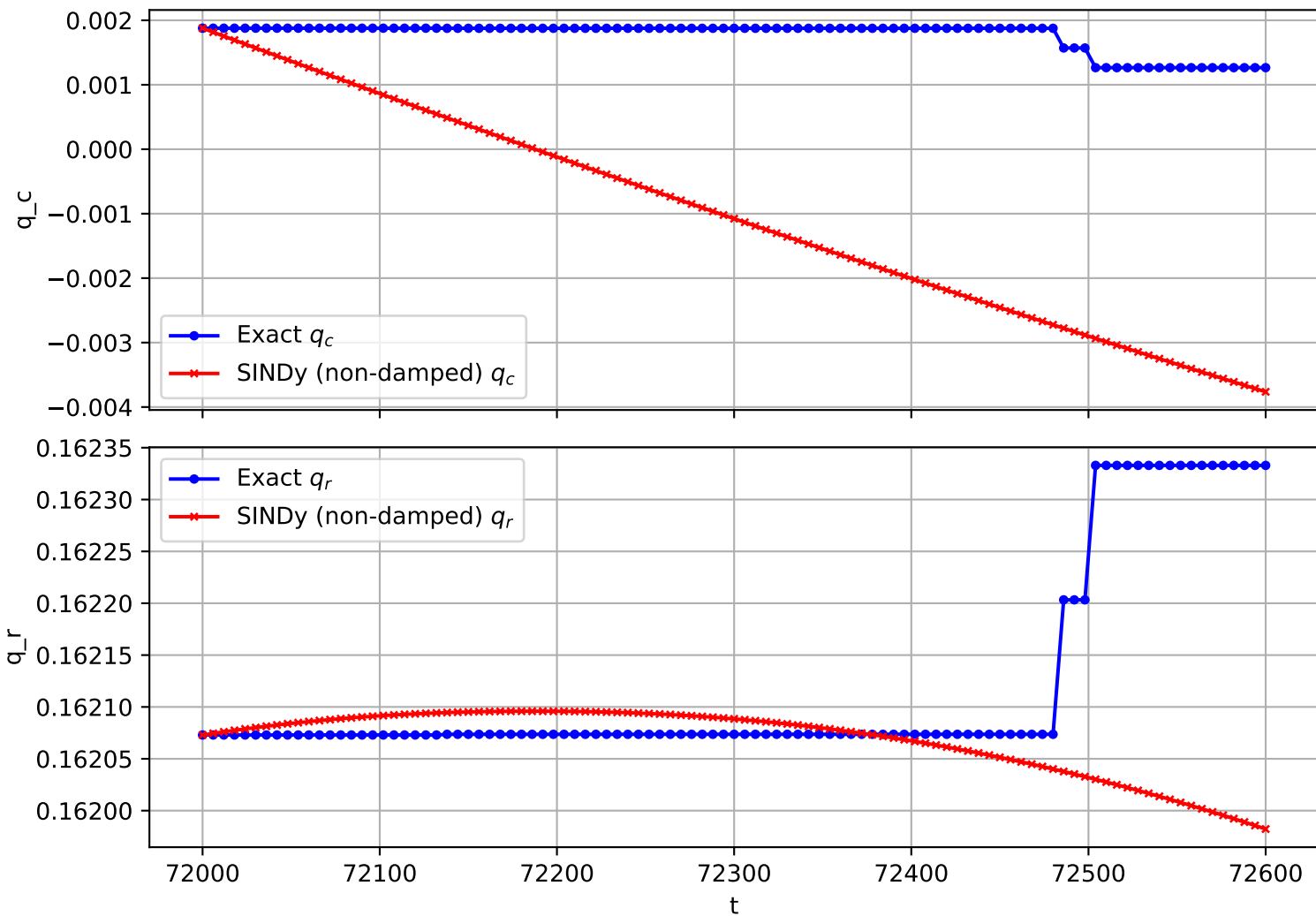
Trajectory 149 (non-damped)
