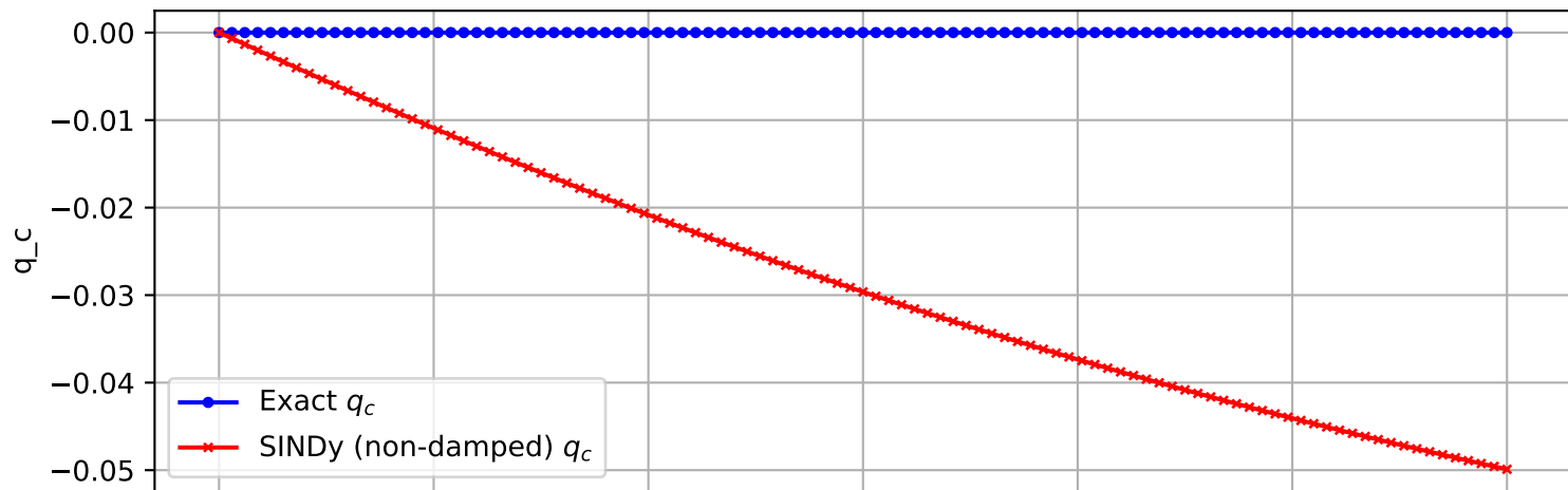
Trajectory 1492 (non-damped)
