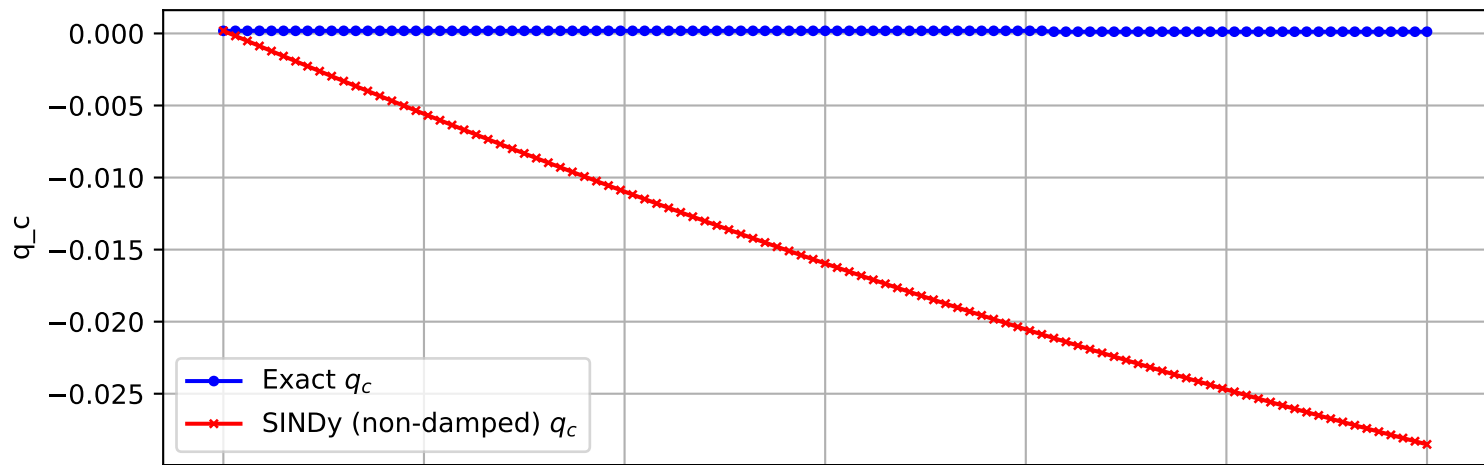
Trajectory 1502 (non-damped)
