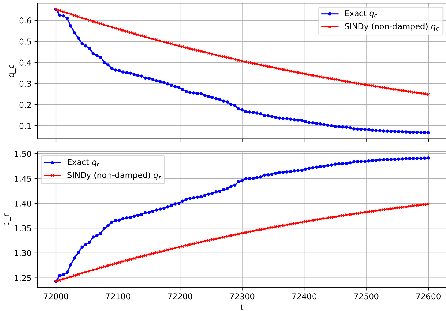
Trajectory 151 (non-damped)
