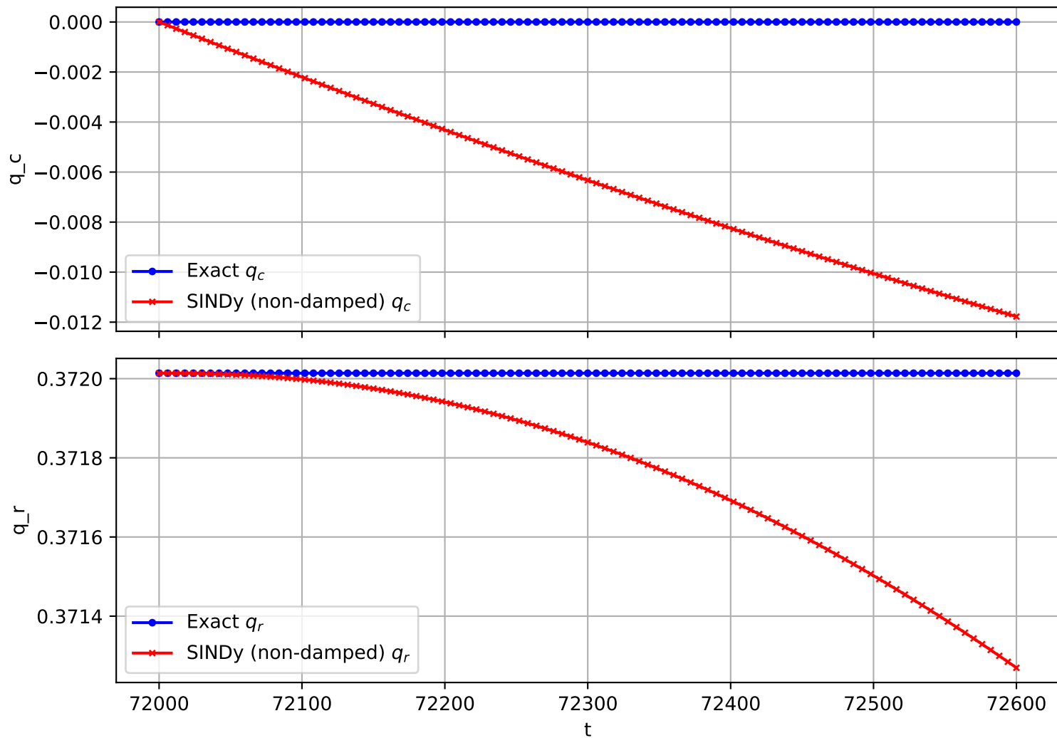
Trajectory 1510 (non-damped)
