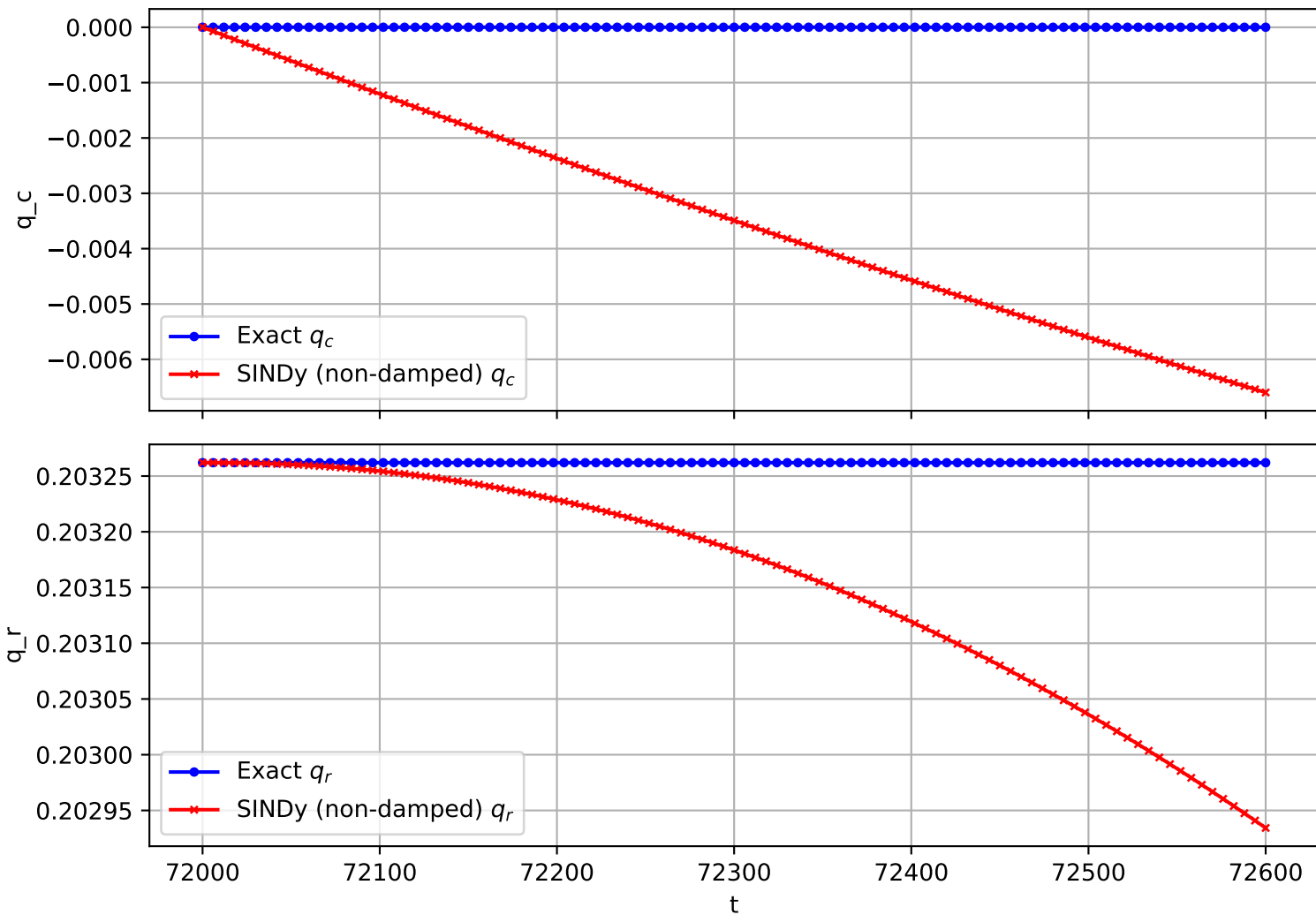
Trajectory 1511 (non-damped)
