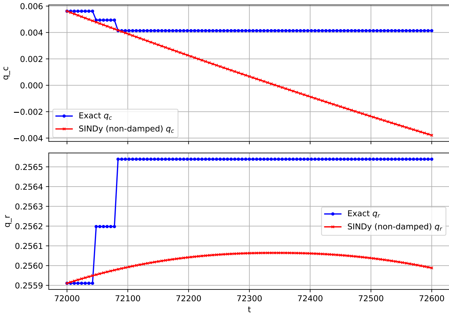
Trajectory 1515 (non-damped)
