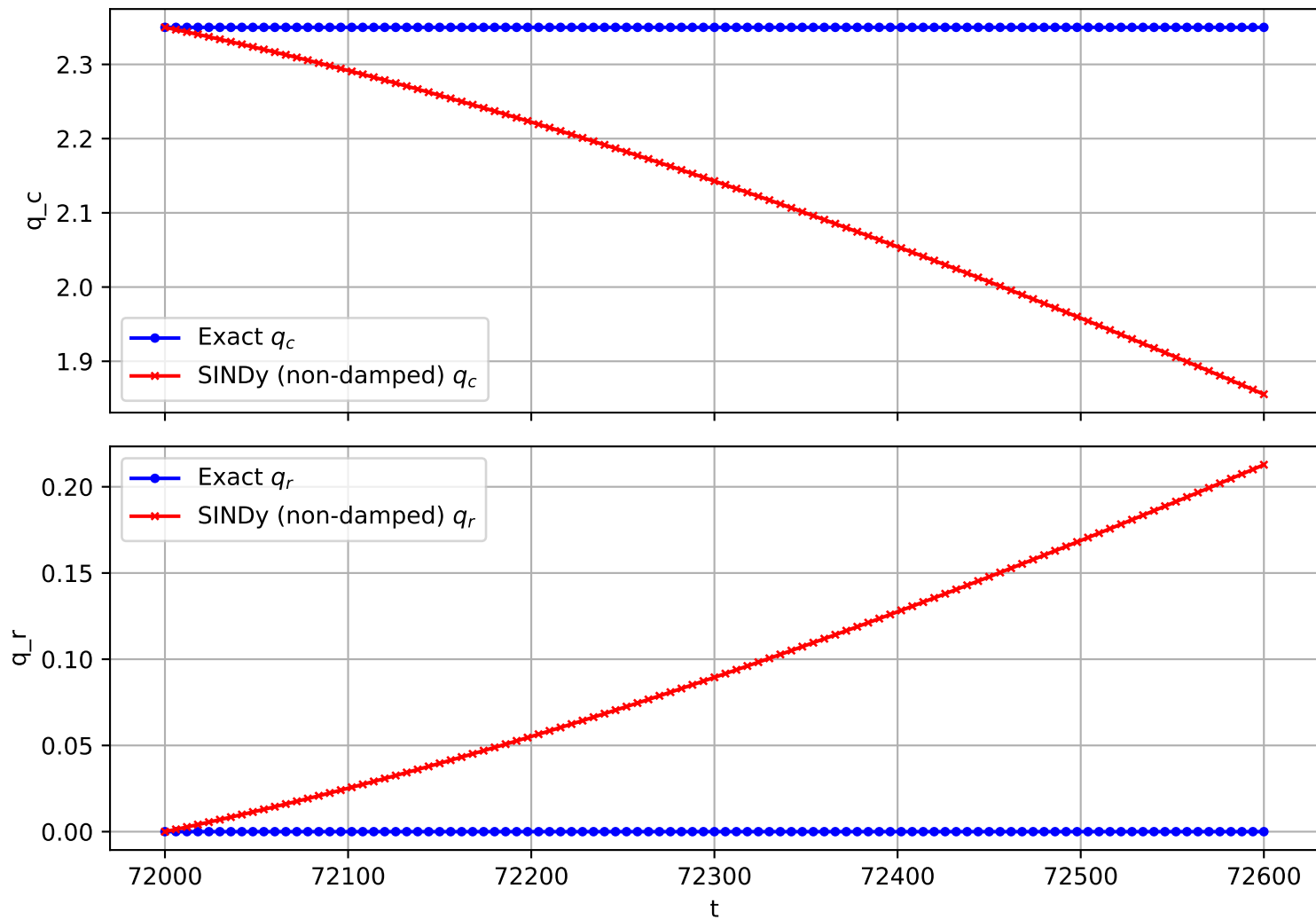
Trajectory 1526 (non-damped)
