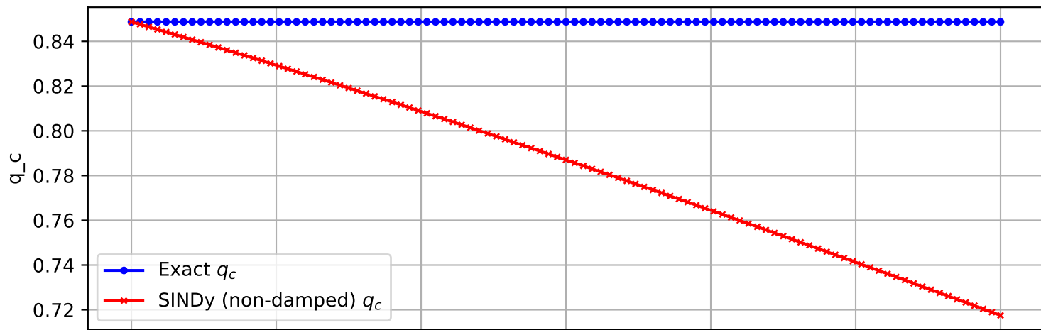
Trajectory 1542 (non-damped)
