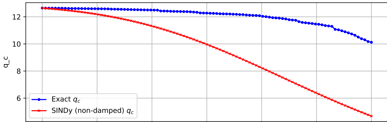
Trajectory 1551 (non-damped)
