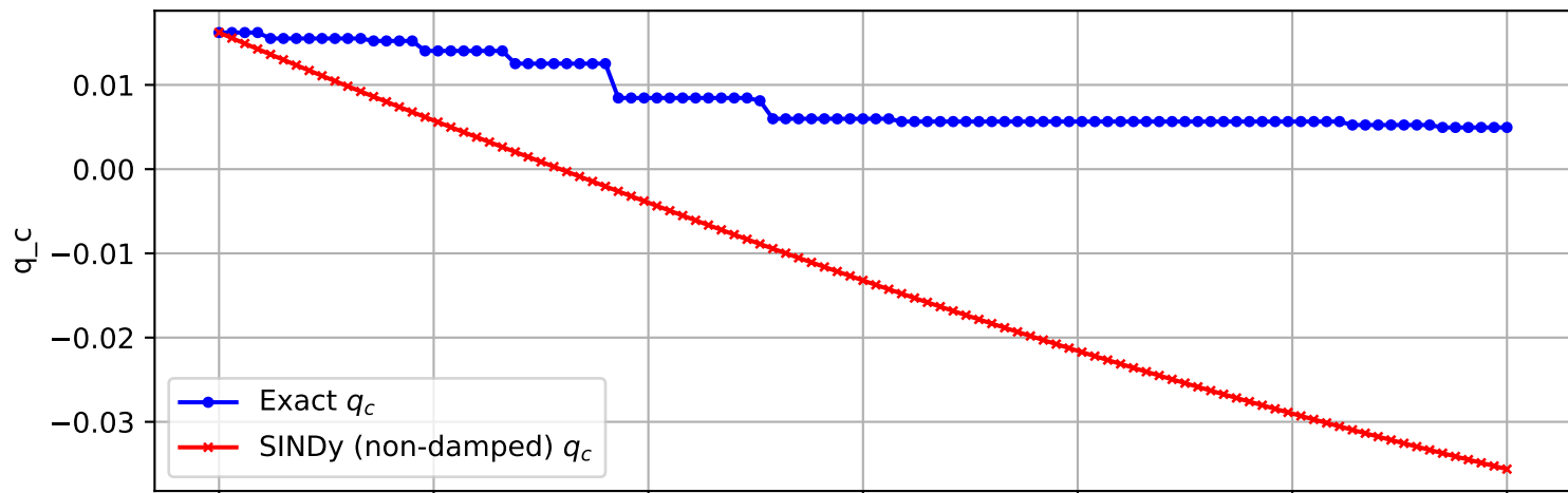
Trajectory 1569 (non-damped)
