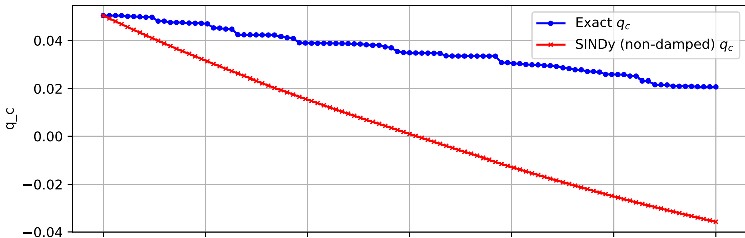
Trajectory 1571 (non-damped)
