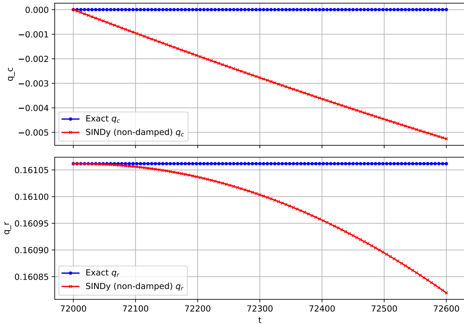
Trajectory 1577 (non-damped)
