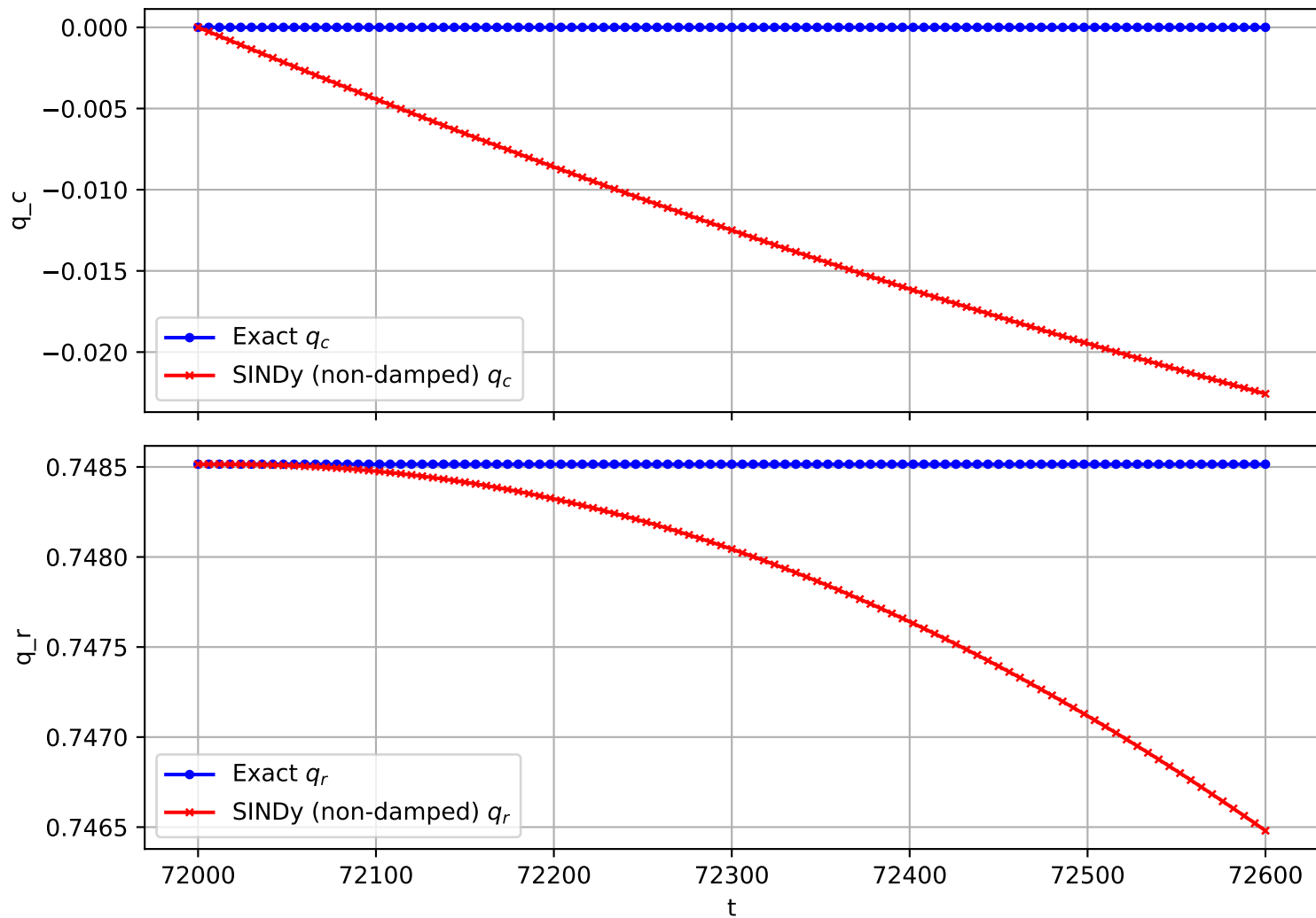
Trajectory 1579 (non-damped)
