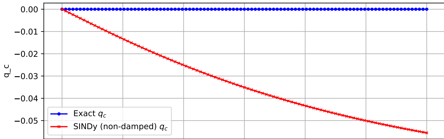
Trajectory 1583 (non-damped)
