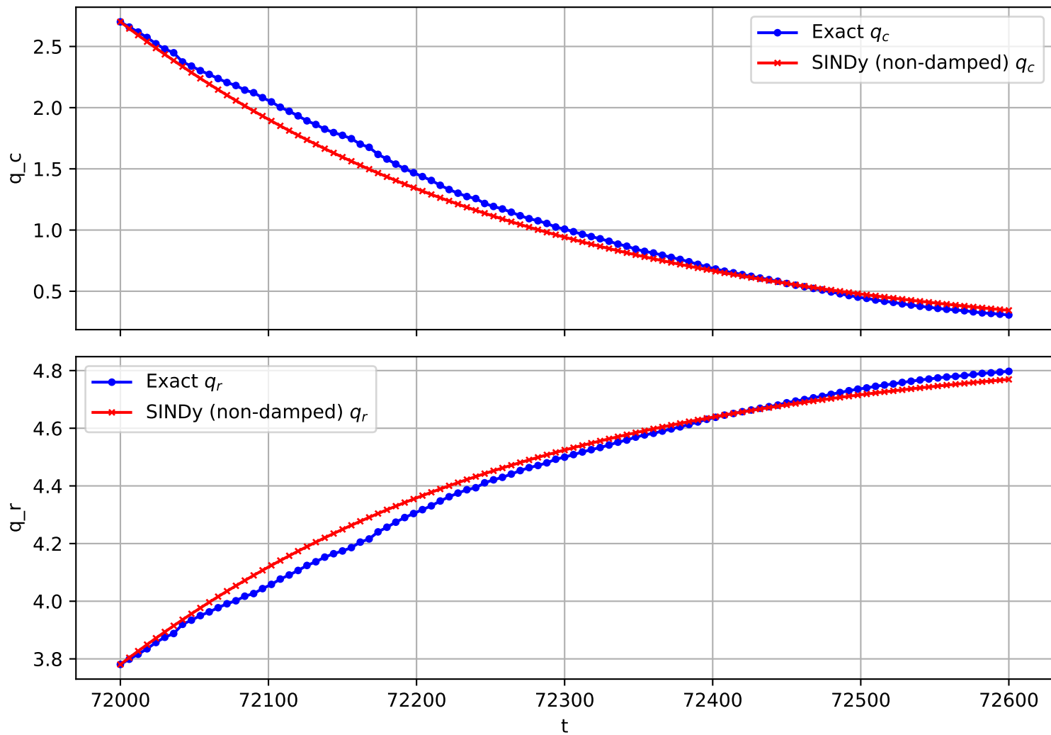
Trajectory 1587 (non-damped)
