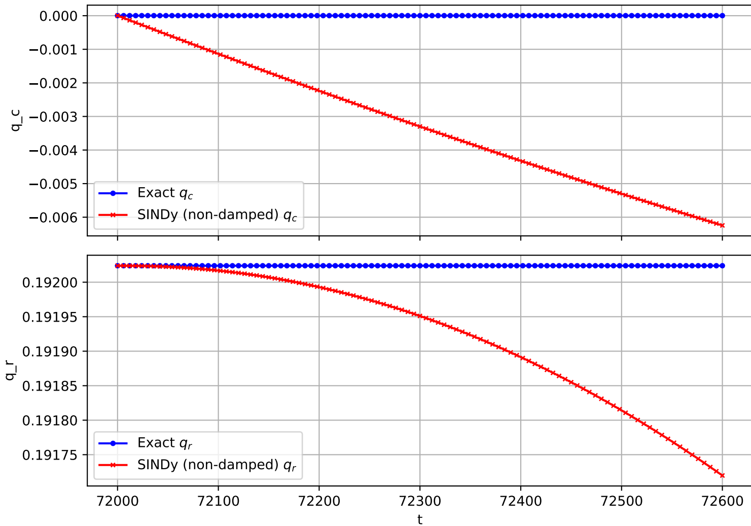
Trajectory 1592 (non-damped)
