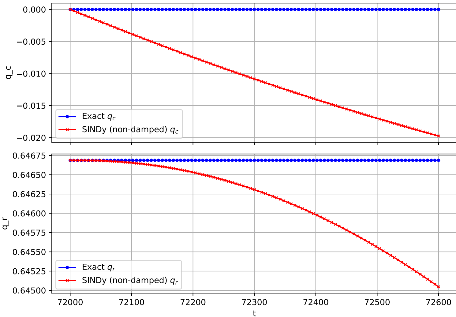
Trajectory 1595 (non-damped)
