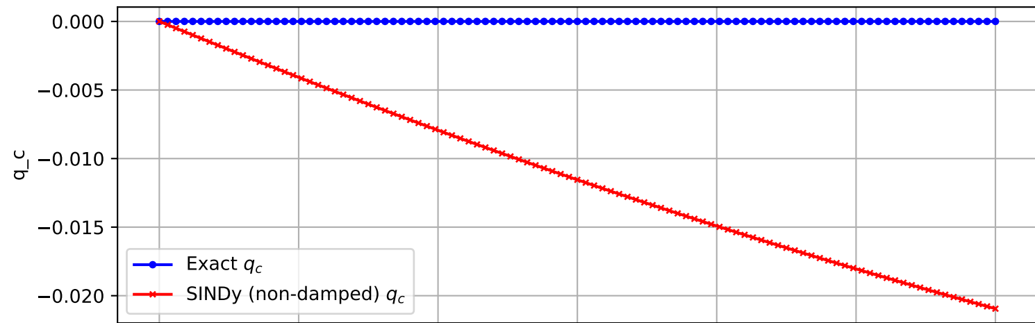
Trajectory 1596 (non-damped)
