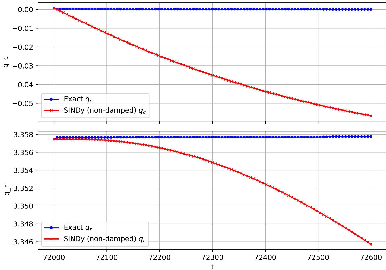
Trajectory 1604 (non-damped)
