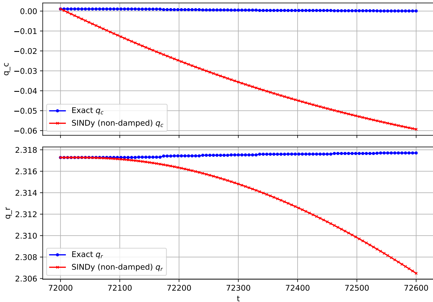
Trajectory 1607 (non-damped)
