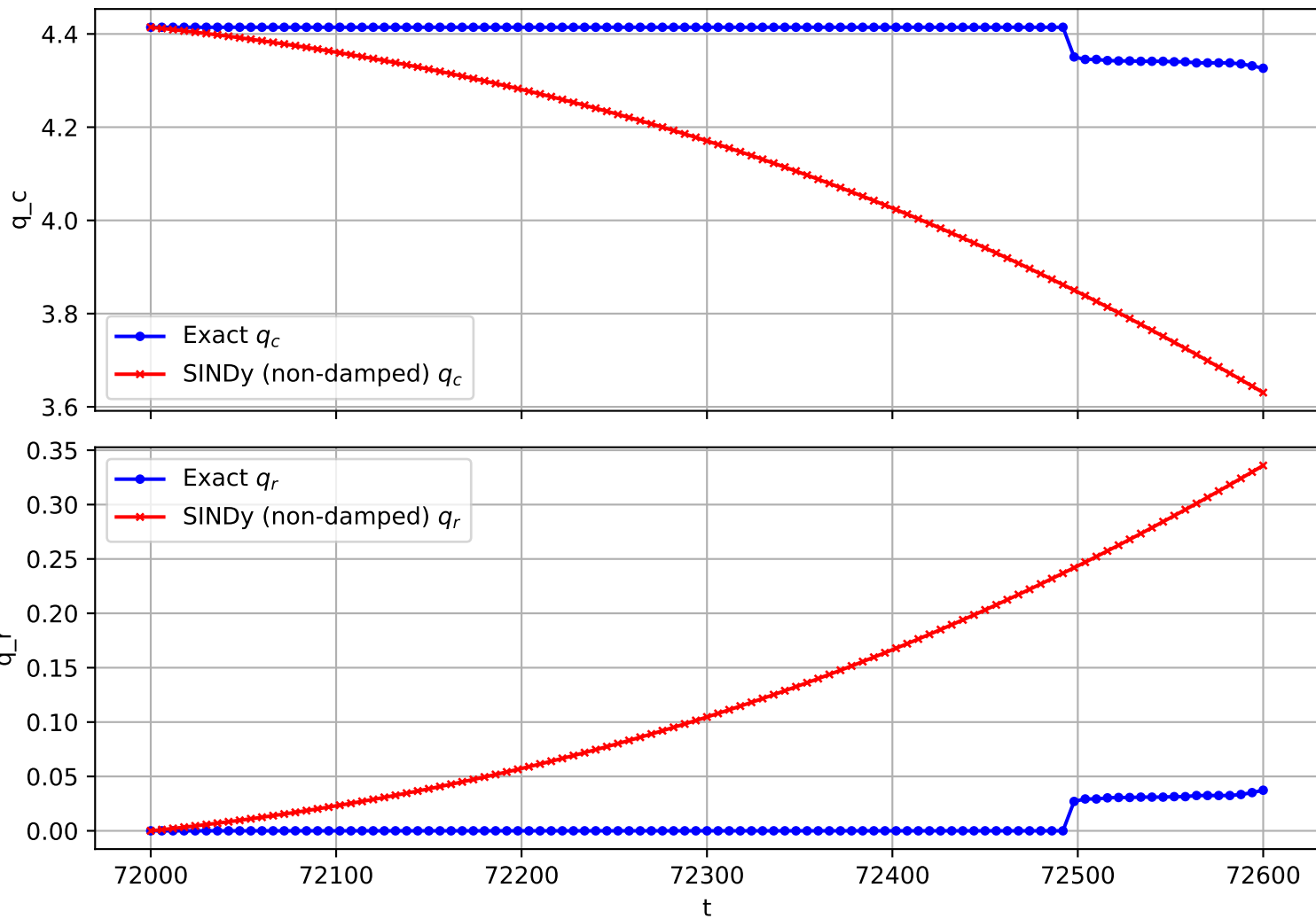
Trajectory 161 (non-damped)
