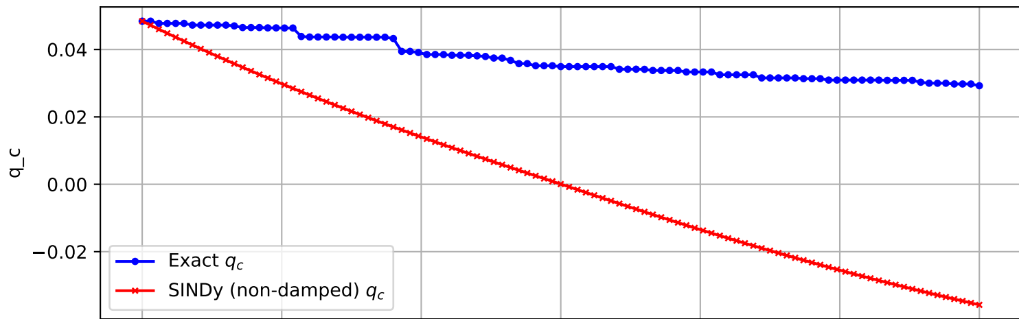
Trajectory 1610 (non-damped)
